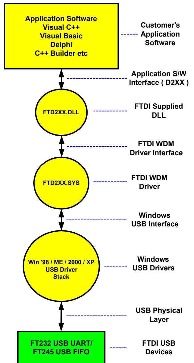
D2XX Driver Architecture
